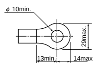
Applicable crimp terminal
