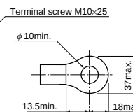
Applicable crimp terminal
